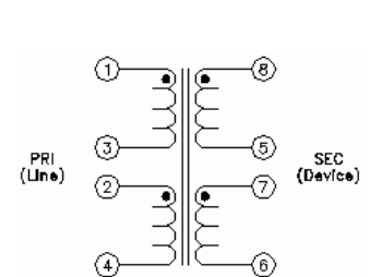
Schematic 1
