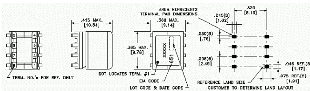
Mechanical 1
