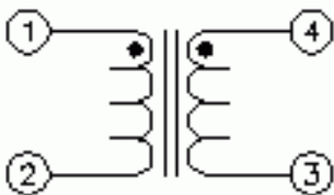
Schematic 1
