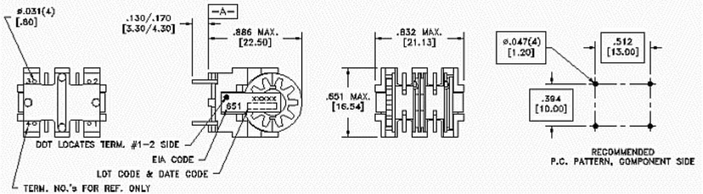
Mechanical 1
